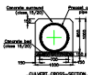
CULVERT CROSS-SECTION
