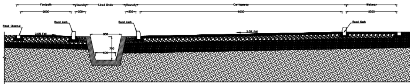
TYPICAL ROAD CROSS-SECTION MATUNDU ROAD
