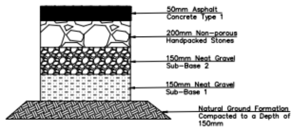
TYPICAL ROAD LAYERS
