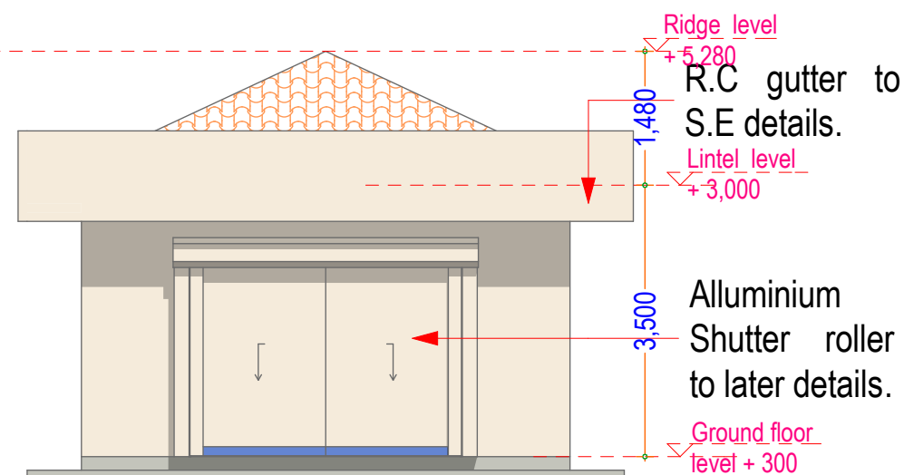
ELEVATION 02 SCALE 1:100
