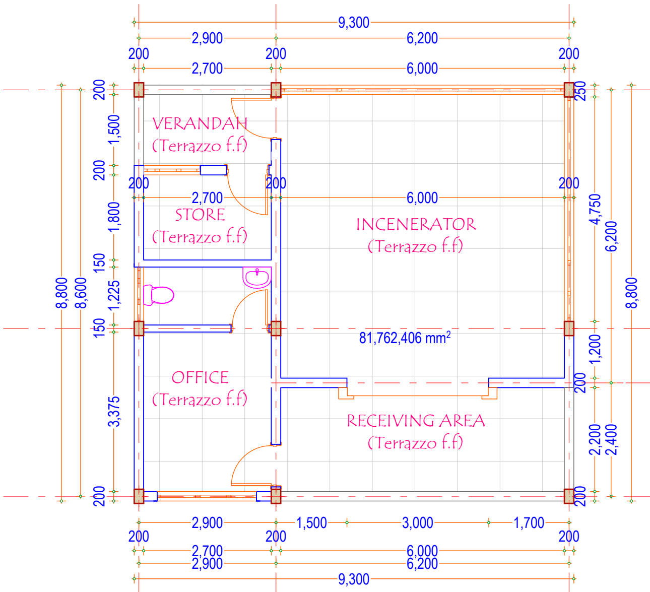
GROUND FLOOR PLAN LAYOUT SCALE 1:100
