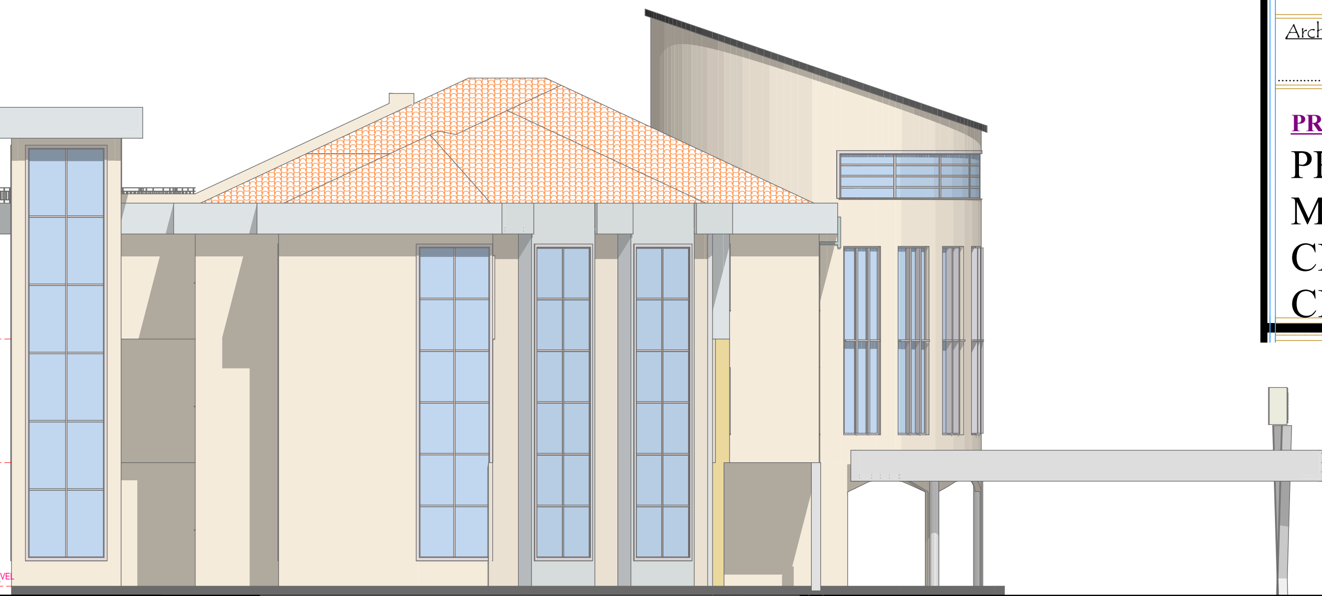
ELEVATION 04 SCALE 1:100
