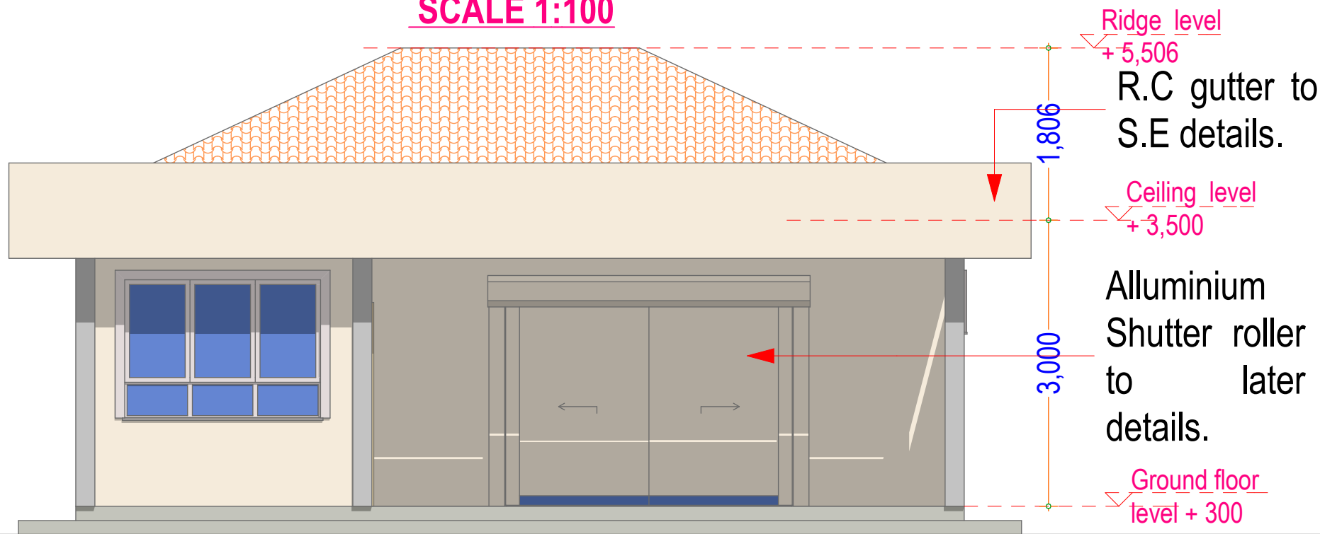
ELEVATION 01 SCALE 1:100
