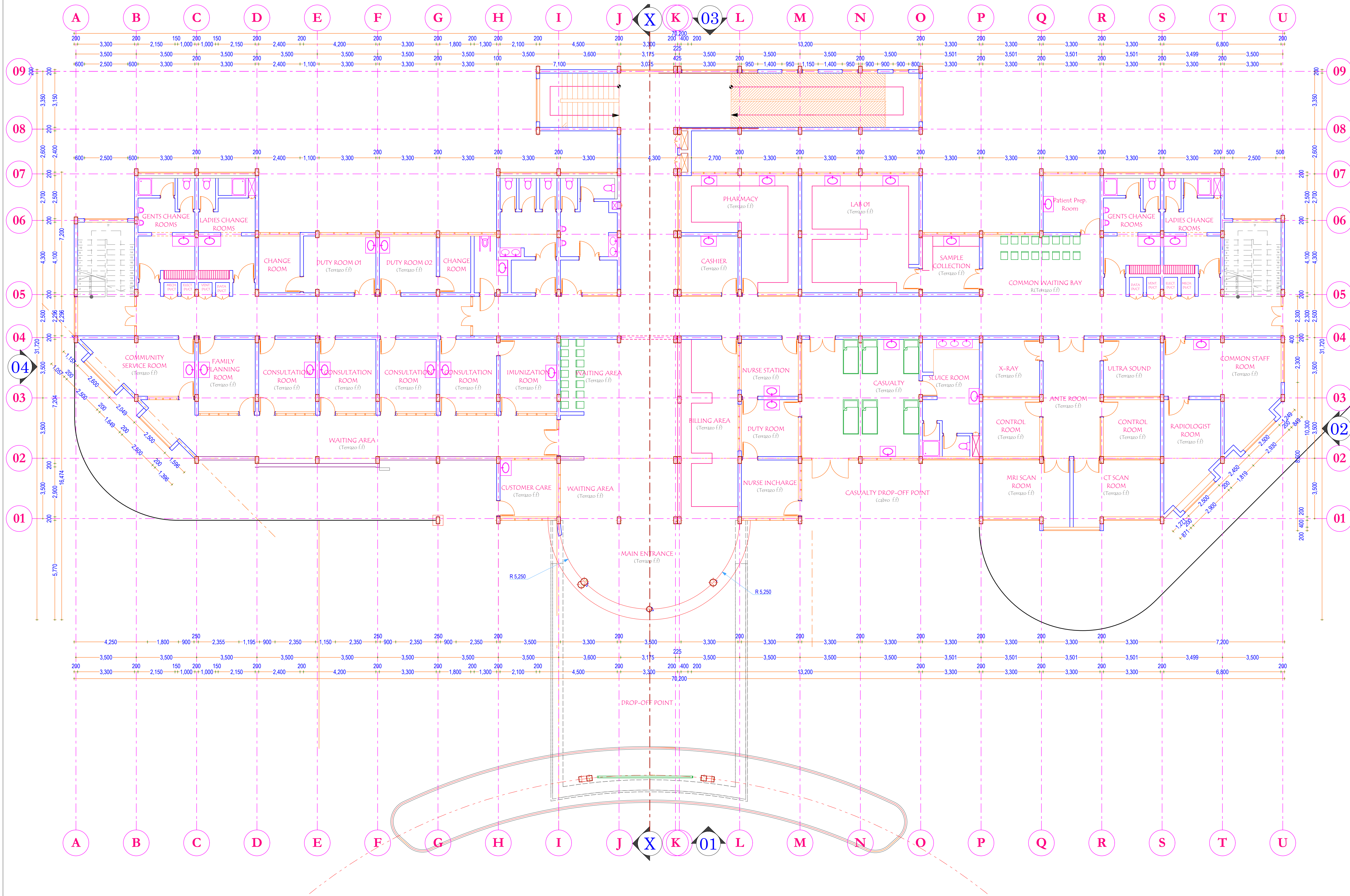
GROUND FLOOR PLAN LAYOUT SCALE 1:100
