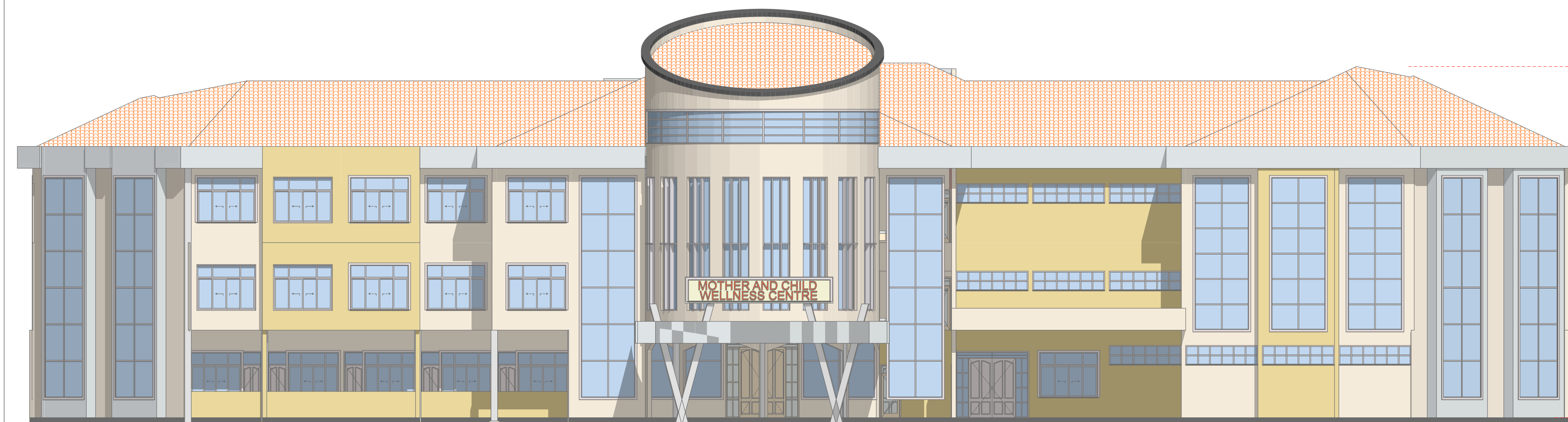
ELEVATION 01 SCALE 1:100
