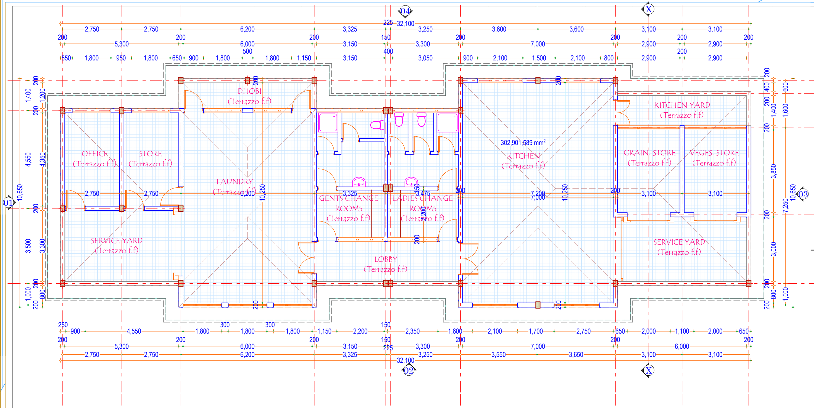
GROUND FLOOR PLAN LAYOUT SCALE 1:100
