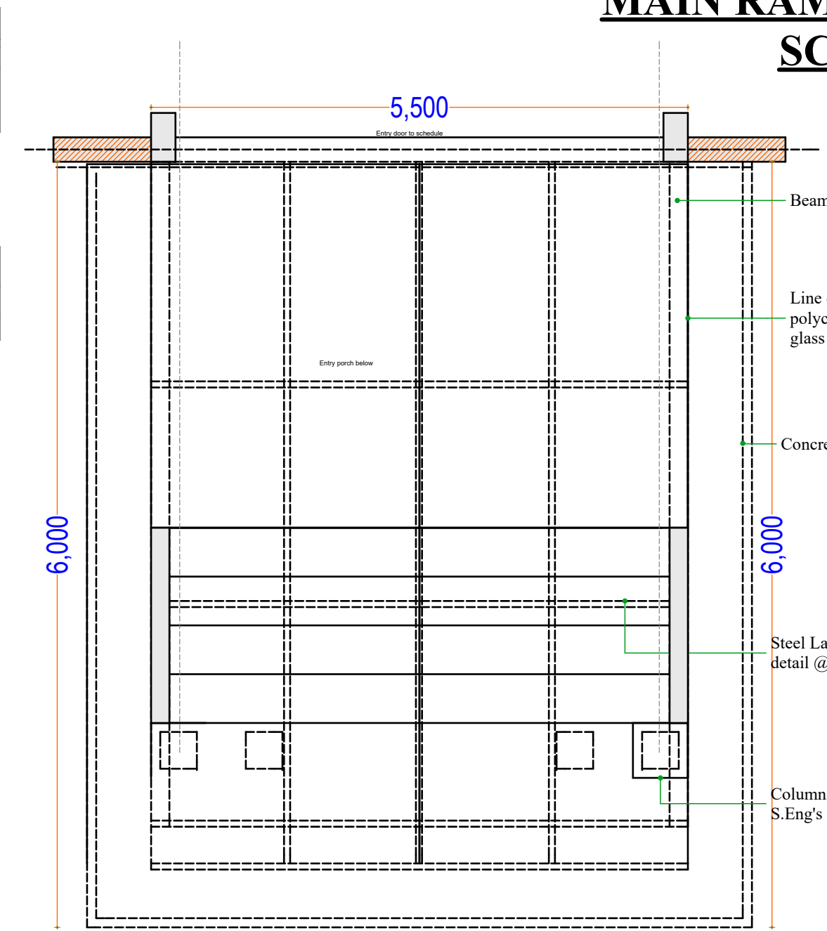
CANOPY PLAN SCALE 1:10
