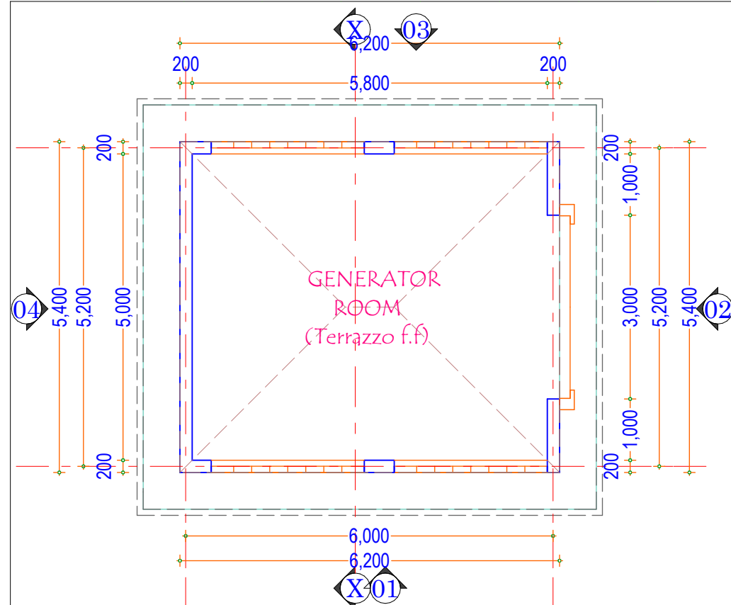
GROUND FLOOR PLAN LAYOUT SCALE 1:100
