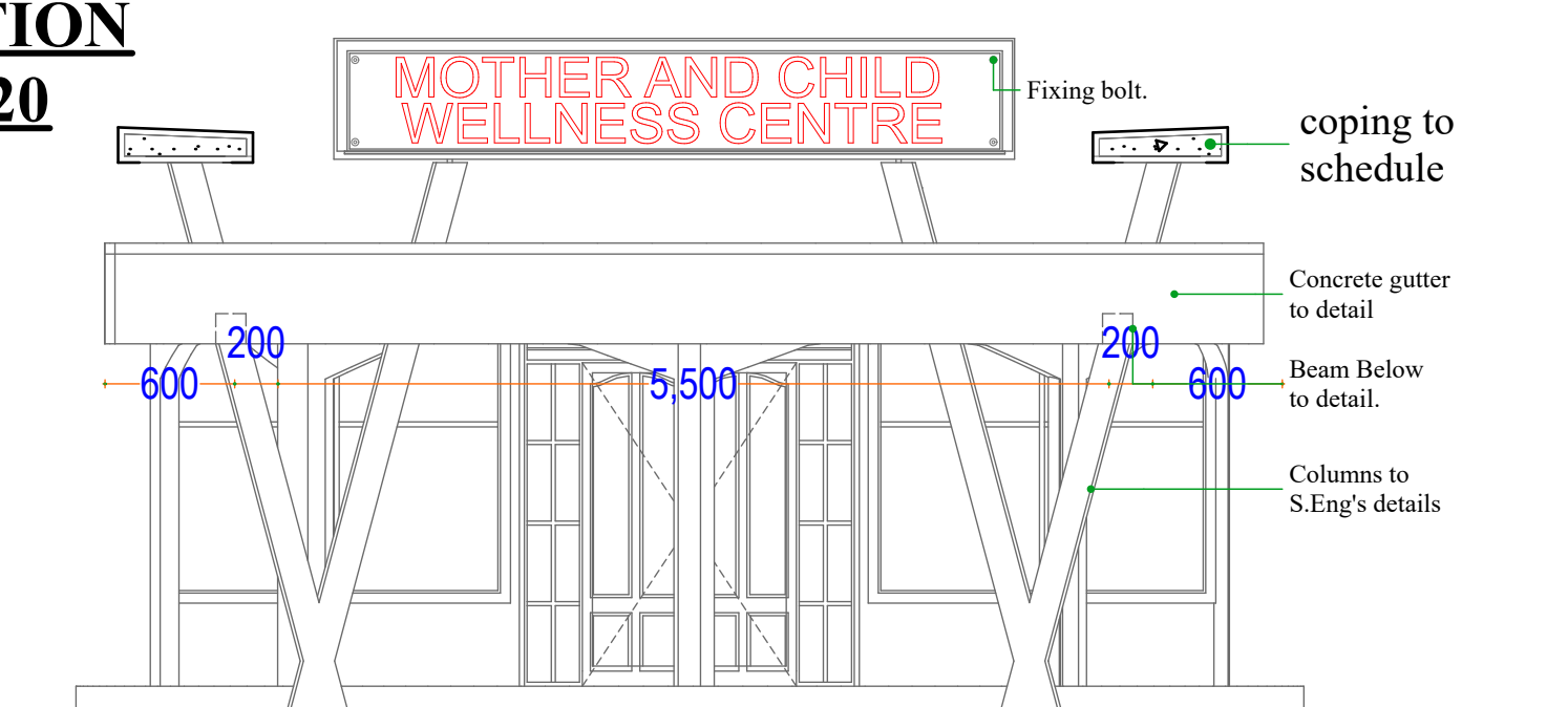
CANOPY ELEVATION SCALE 1:10
