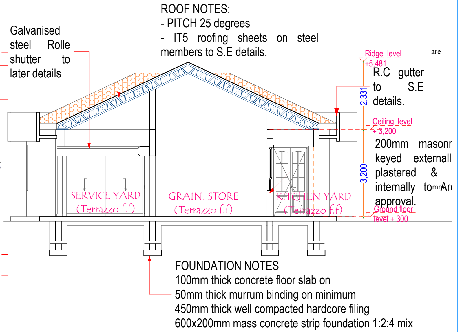
SECTION X-X SCALE 1:100
