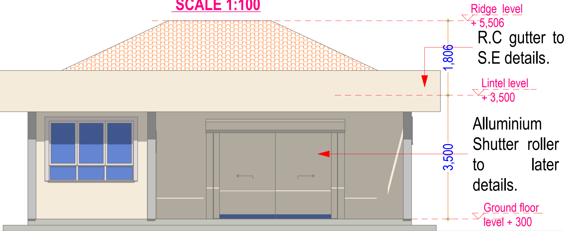
ELEVATION 01 SCALE 1:100
