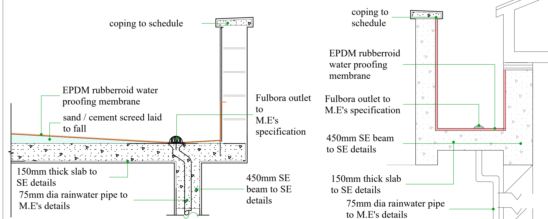
FLAT ROOF DETAIL SCALE 1:10
