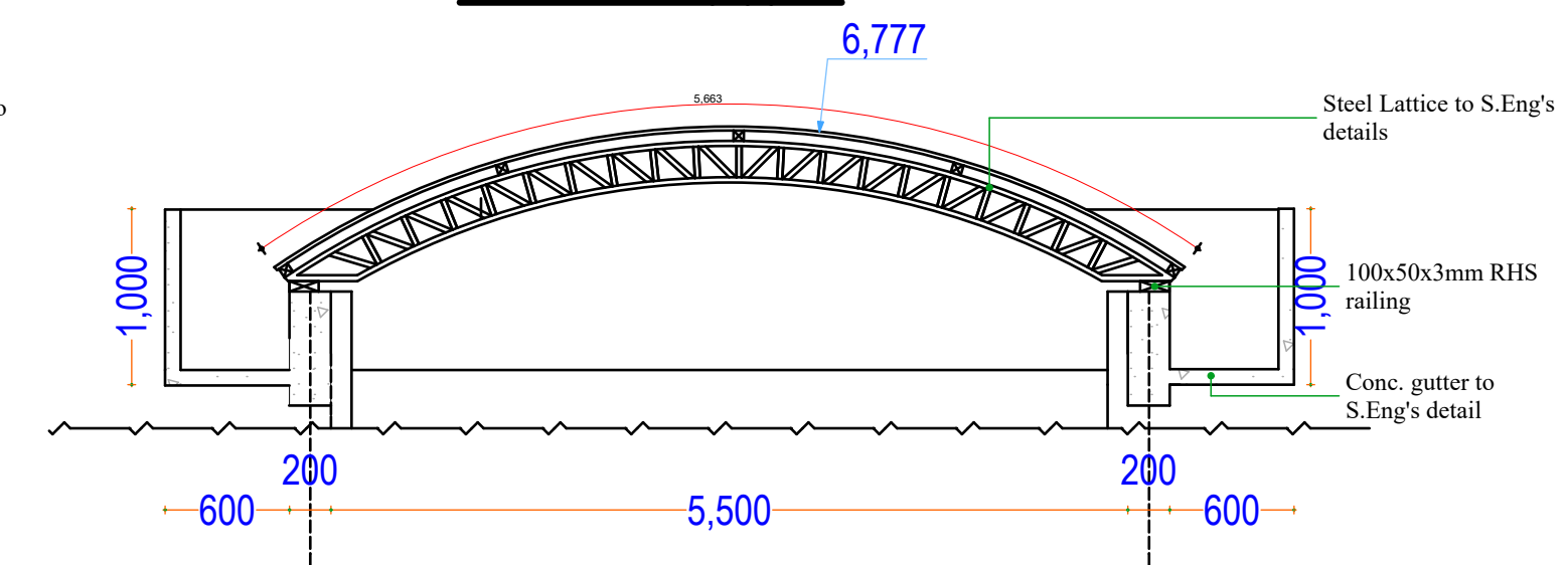
CANOPY SECTION SCALE 1:10
