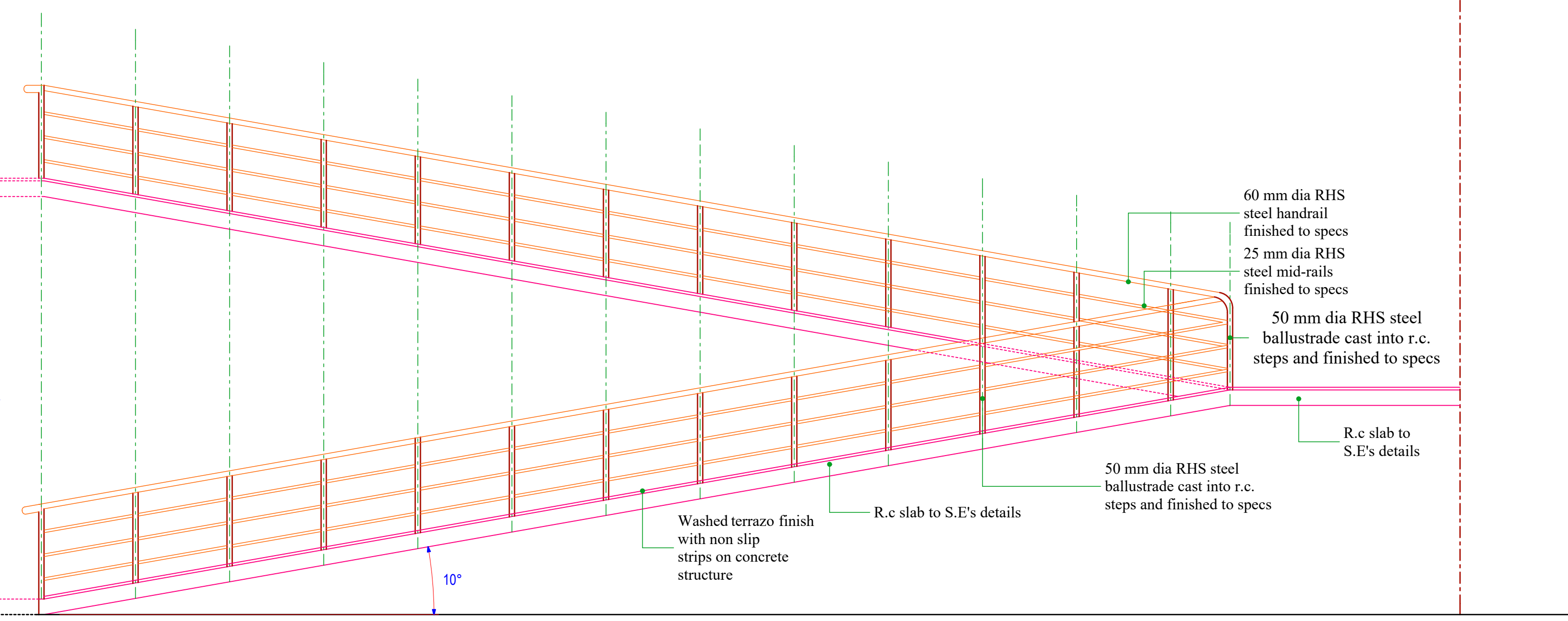
MAIN RAMP SECTION SCALE 1:20
