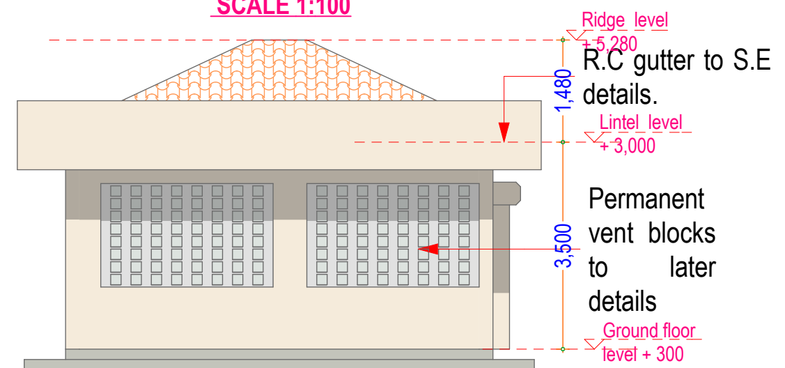
ELEVATION 01 SCALE 1:100
