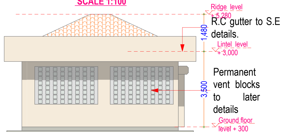
ELEVATION 01 SCALE 1:100
