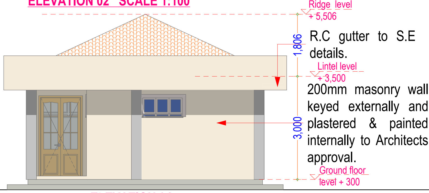
ELEVATION 04 SCALE 1:100
