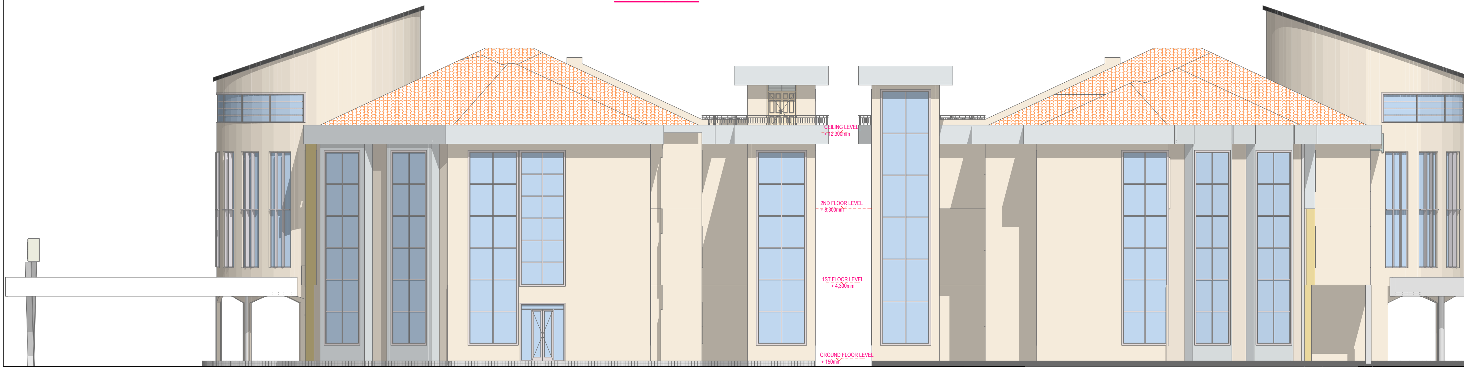
ELEVATION 02 SCALE 1:100
