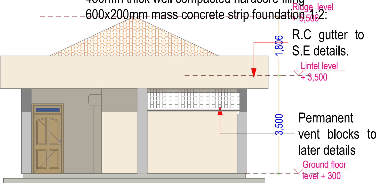
ELEVATION 02 SCALE 1:100
