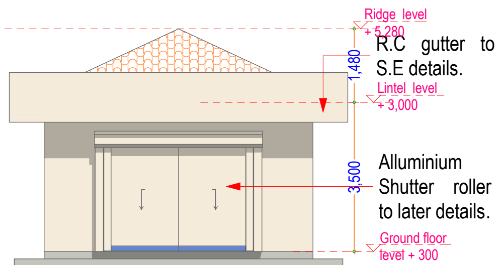
ELEVATION 02 SCALE 1:100
